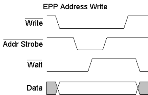
Figure 2. Enhanced Parallel Port Address Write Cycle.
