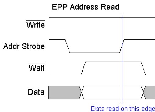
Figure 4. Enhanced Parallel Port Address Read Cycle.
