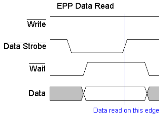
Figure 3. Enhanced Parallel Port Data Read Cycle.
